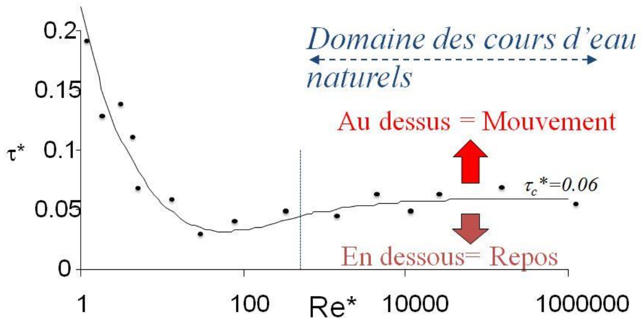
Figure 16: La courbe de Shields
